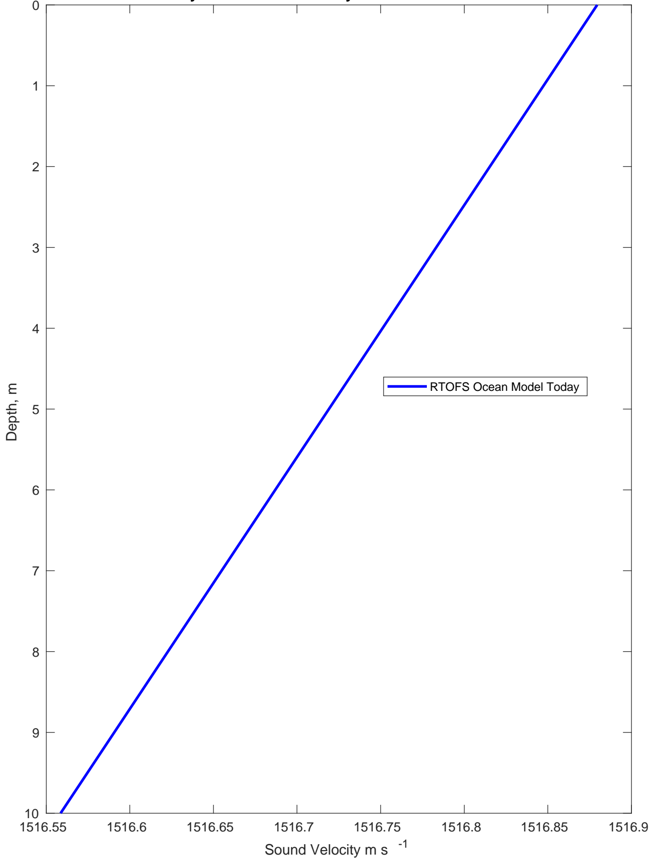
Sound Velocity Profile for TABS Buoy D on 08-Dec-2020 00:00:00
